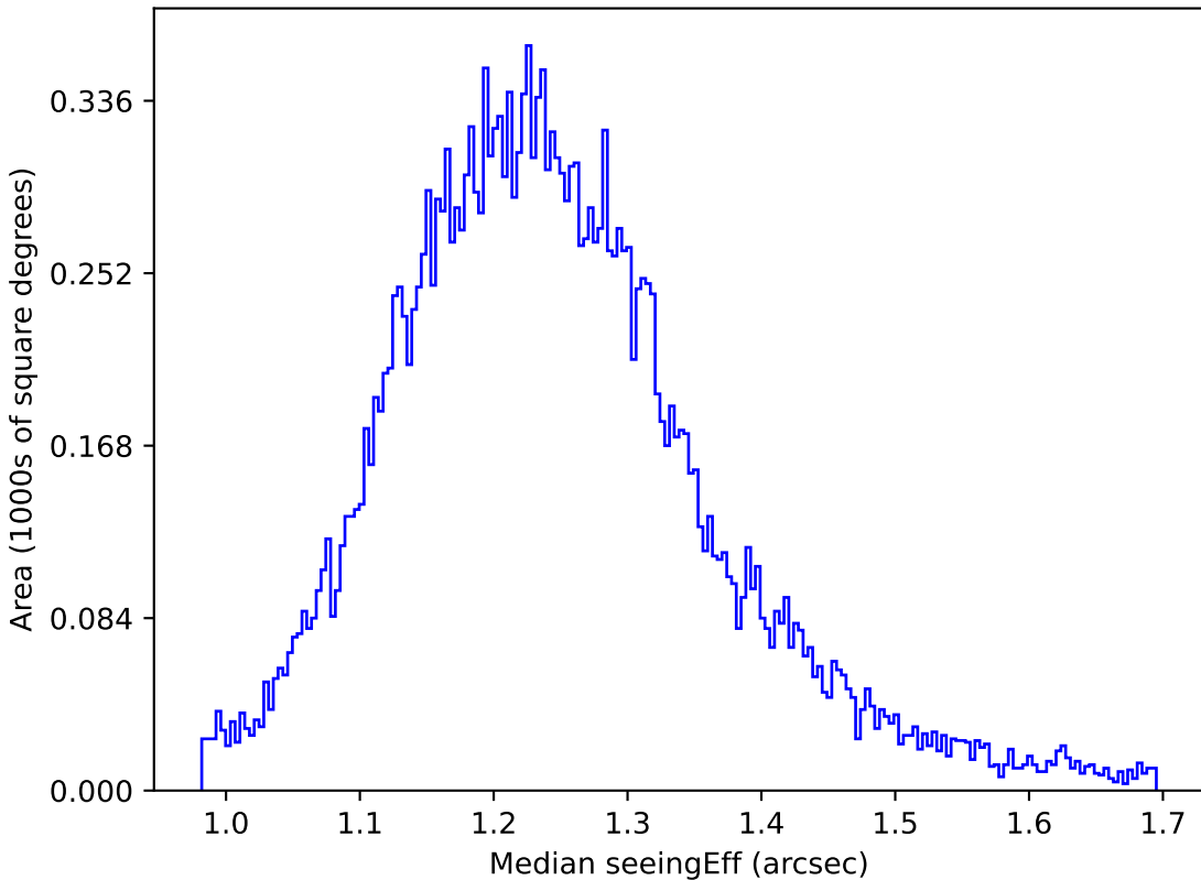
too_5_1v3.4_10yrs All sky u band: Median seeingEff
