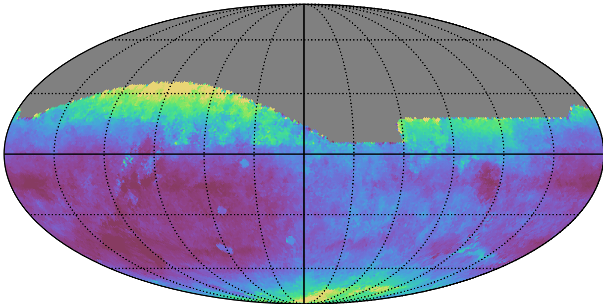
too_5_1v3.4_10yrs All sky r band: Median seeingEff
