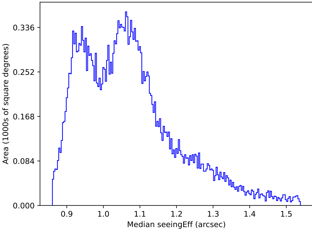
too_5_1v3.4_10yrs All sky r band: Median seeingEff
