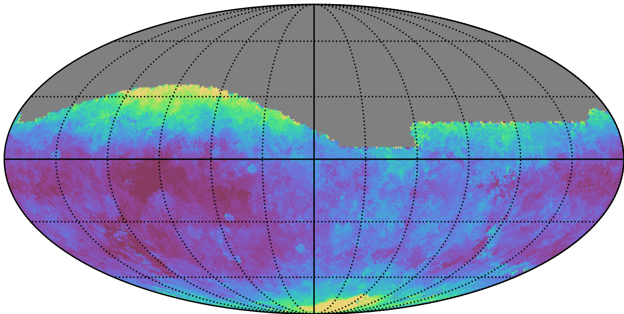
too_5_1v3.4_10yrs All sky g band: Median seeingEff
