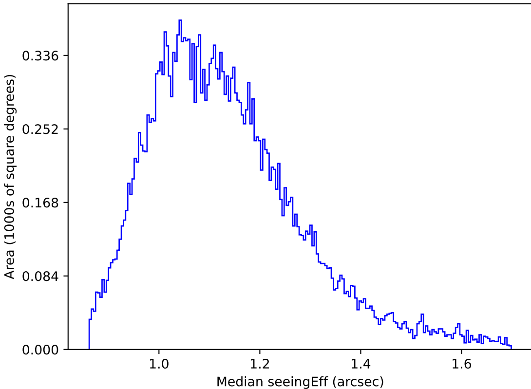
too_5_1v3.4_10yrs All sky g band: Median seeingEff
