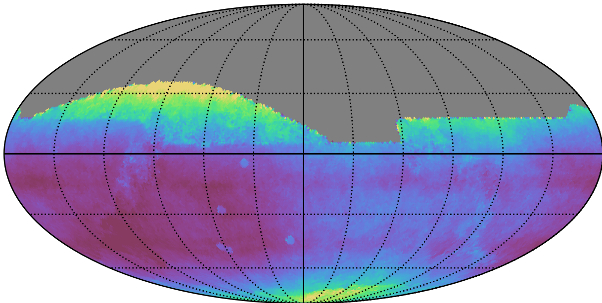
too_5_1v3.4_10yrs All sky all bands: Median seeingEff
