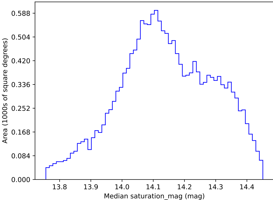
too_5_1v3.4_10yrs WFD z band: Median saturation_mag
