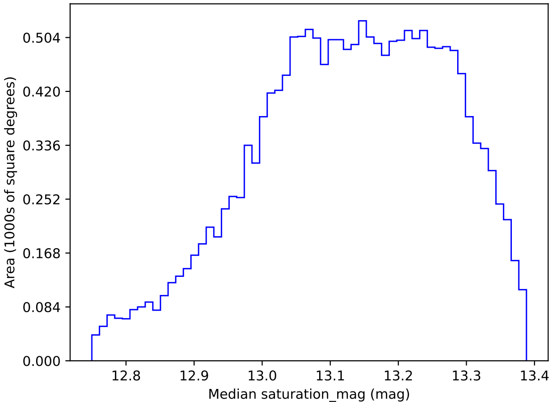
too_5_1v3.4_10yrs WFD y band: Median saturation_mag
