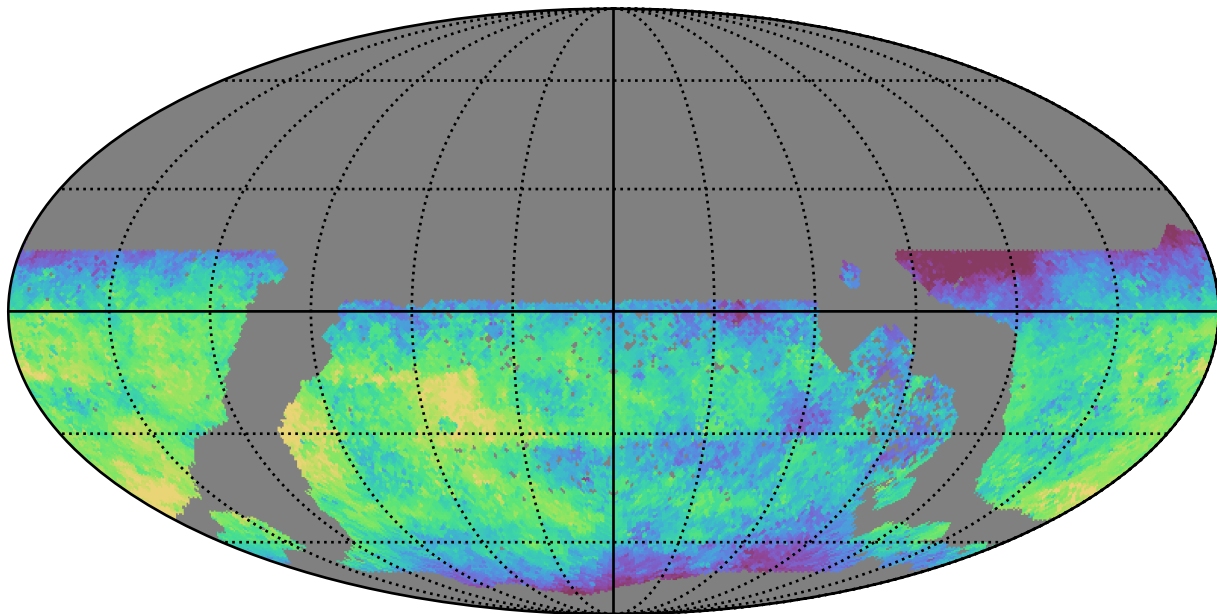
too_5_1v3.4_10yrs WFD u band: Median saturation_mag
