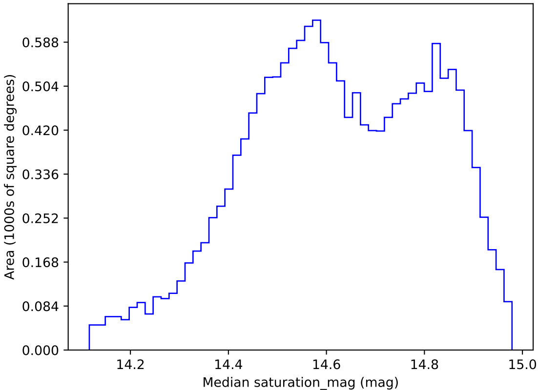
too_5_1v3.4_10yrs WFD r band: Median saturation_mag
