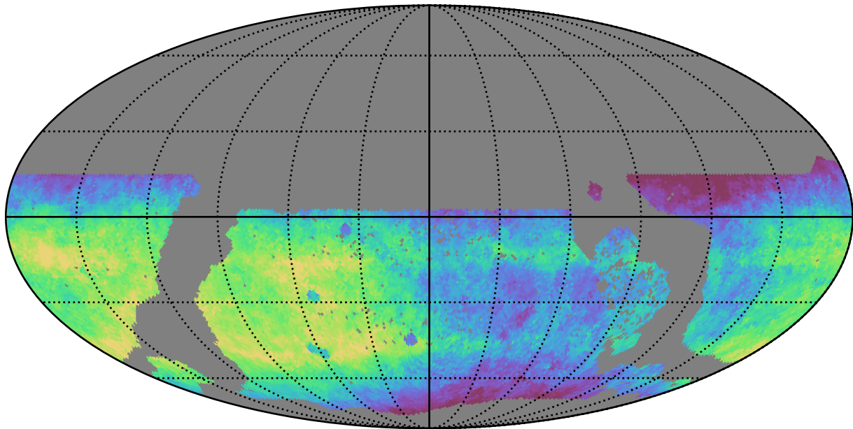
too_5_1v3.4_10yrs WFD i band: Median saturation_mag
