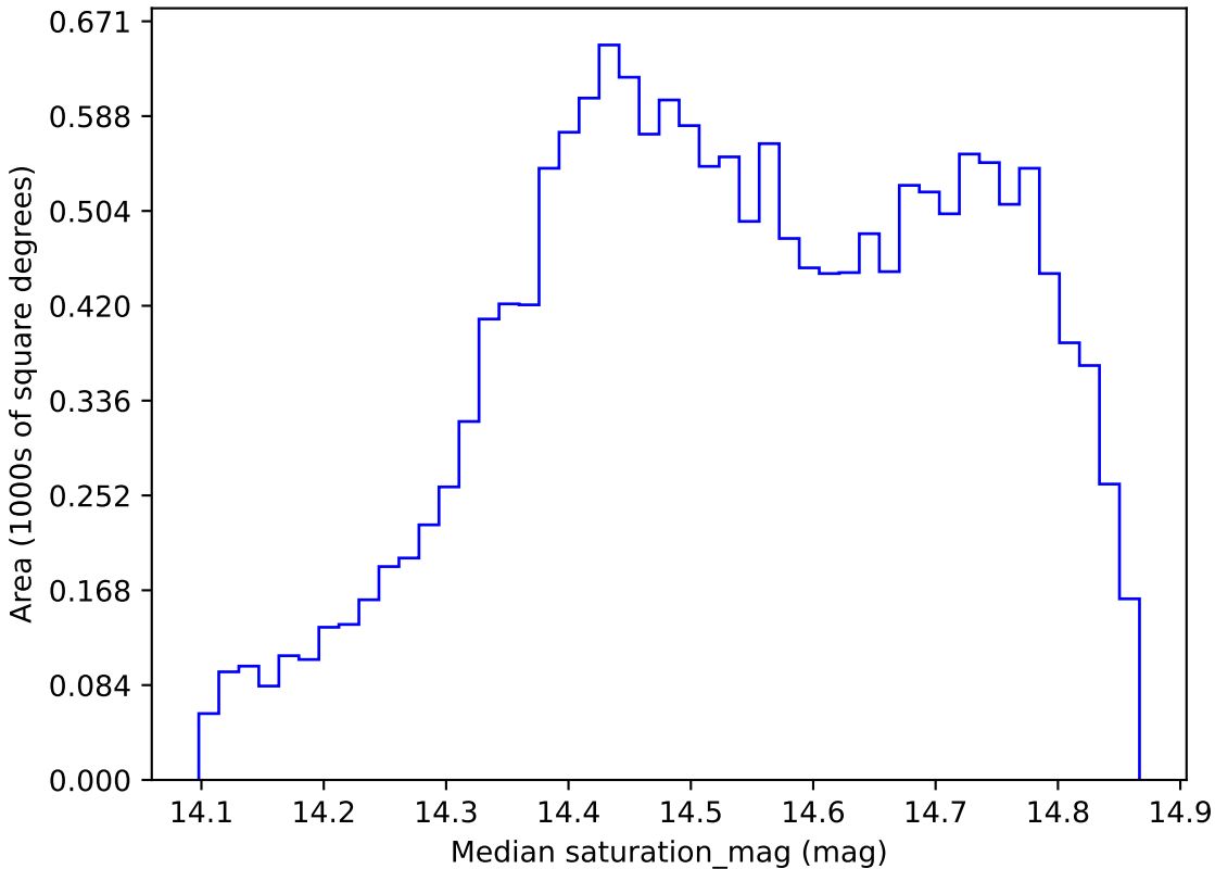
too_5_1v3.4_10yrs WFD i band: Median saturation_mag
