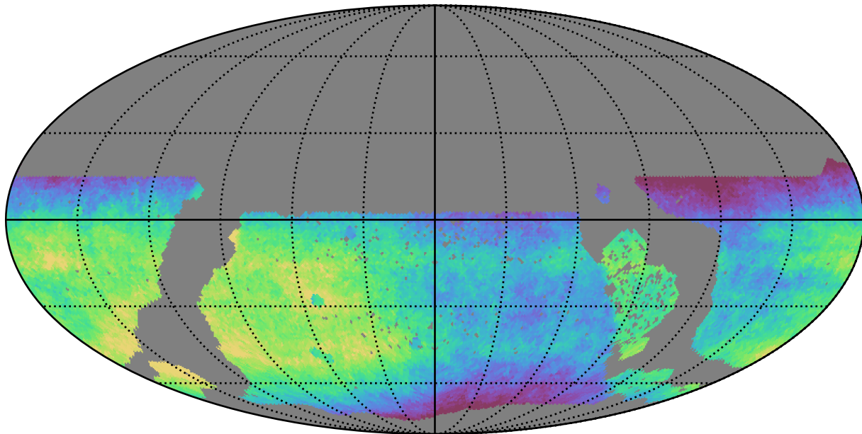
too_5_1v3.4_10yrs WFD all bands: Median saturation_mag
