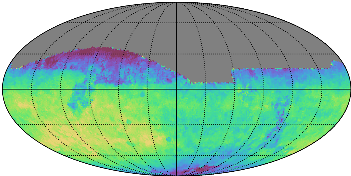
too_5_1v3.4_10yrs All sky z band: Median saturation_mag
