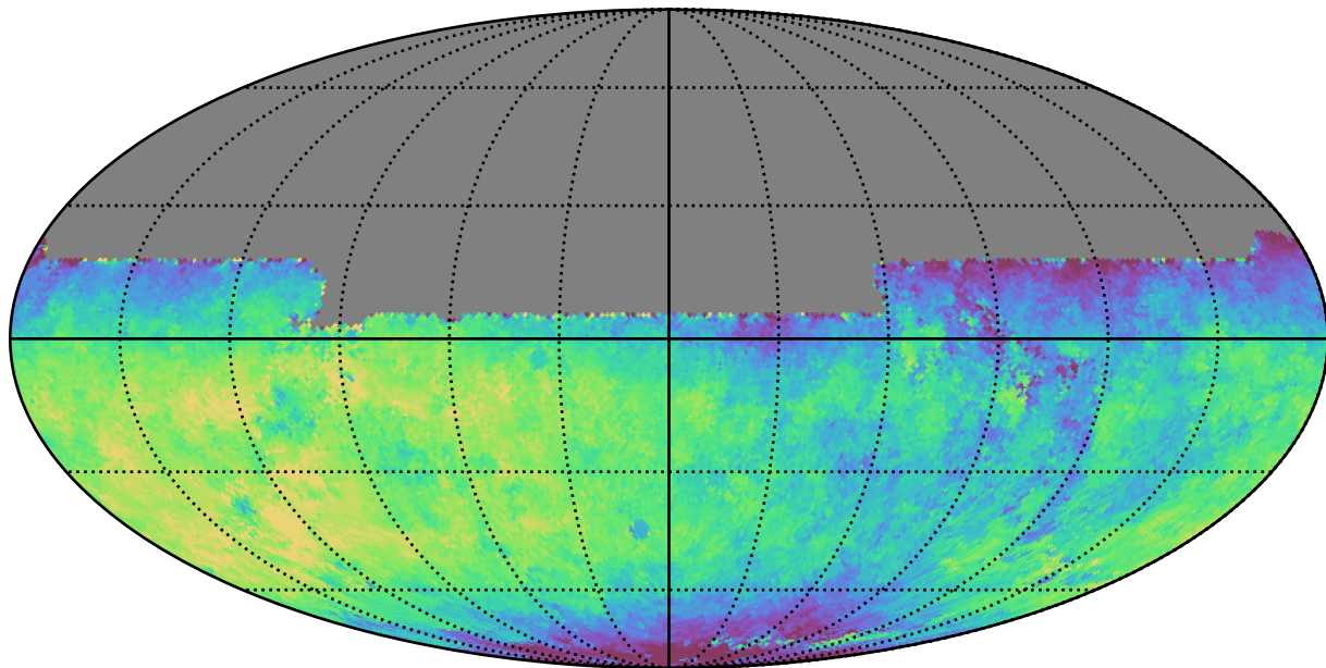
too_5_1v3.4_10yrs All sky y band: Median saturation_mag
