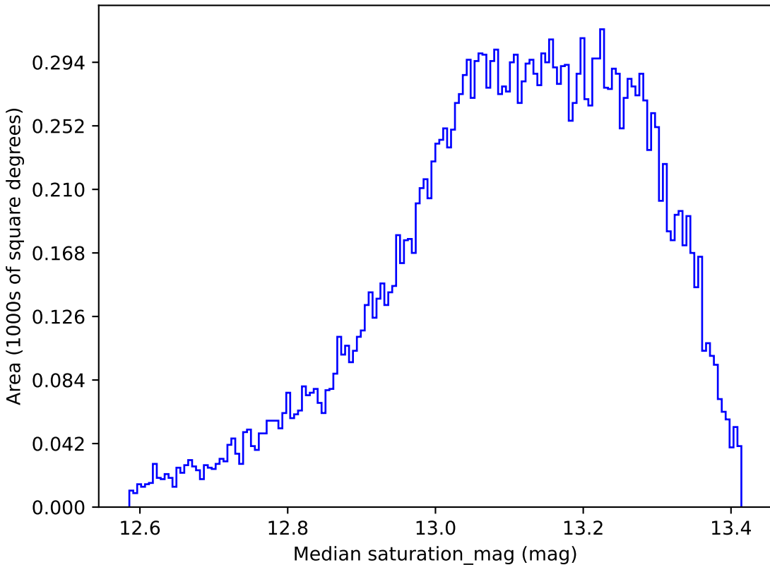
too_5_1v3.4_10yrs All sky y band: Median saturation_mag
