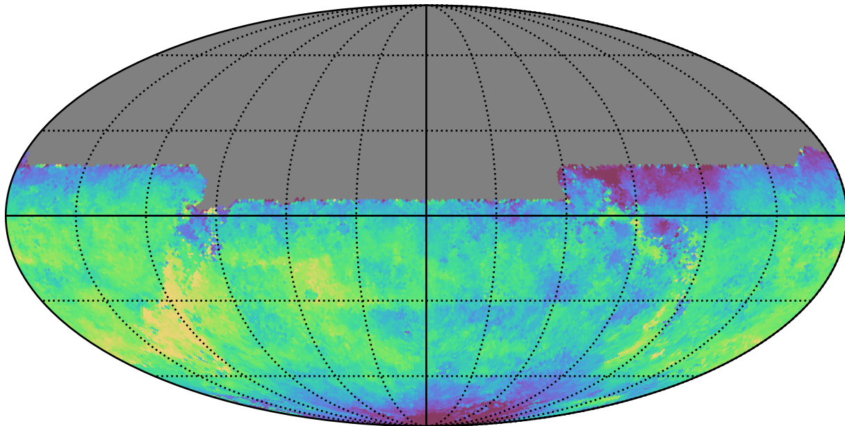
too_5_1v3.4_10yrs All sky u band: Median saturation_mag
