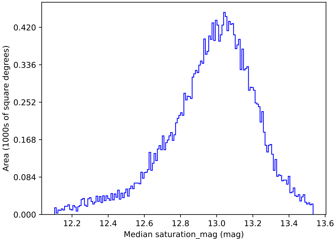
too_5_1v3.4_10yrs All sky u band: Median saturation_mag
