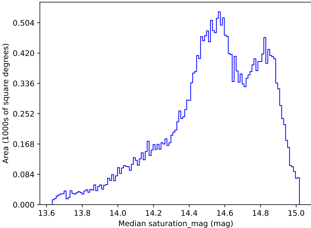
too_5_1v3.4_10yrs All sky r band: Median saturation_mag
