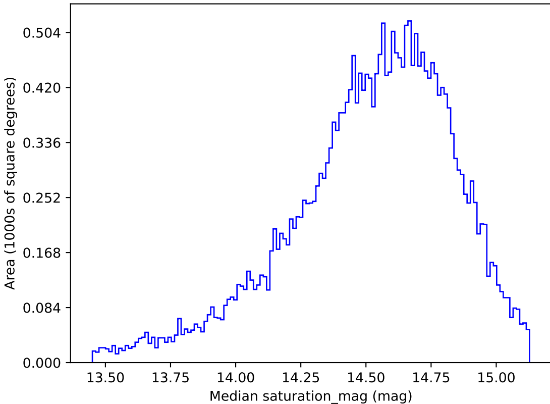
too_5_1v3.4_10yrs All sky g band: Median saturation_mag
