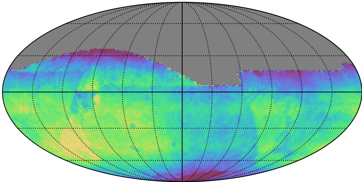
too_5_1v3.4_10yrs All sky all bands: Median saturation_mag
