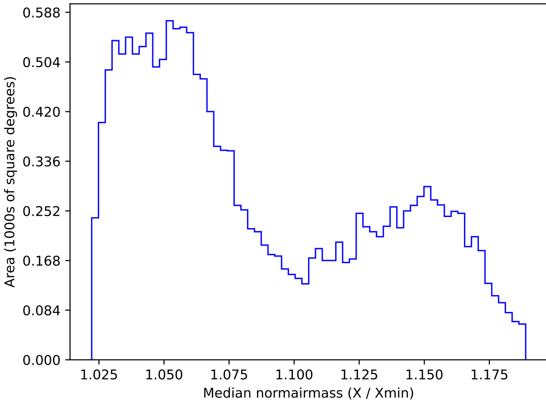
too_5_1v3.4_10yrs WFD z band: Median normairmass
