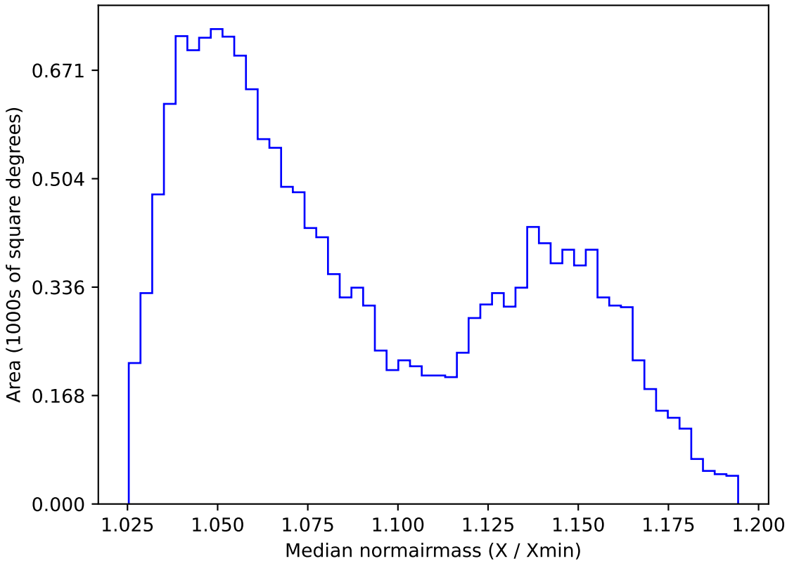
too_5_1v3.4_10yrs WFD y band: Median normairmass
