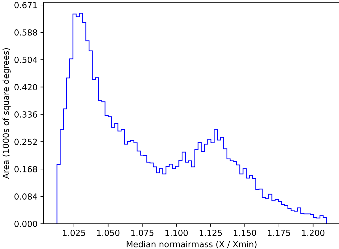
too_5_1v3.4_10yrs WFD u band: Median normairmass
