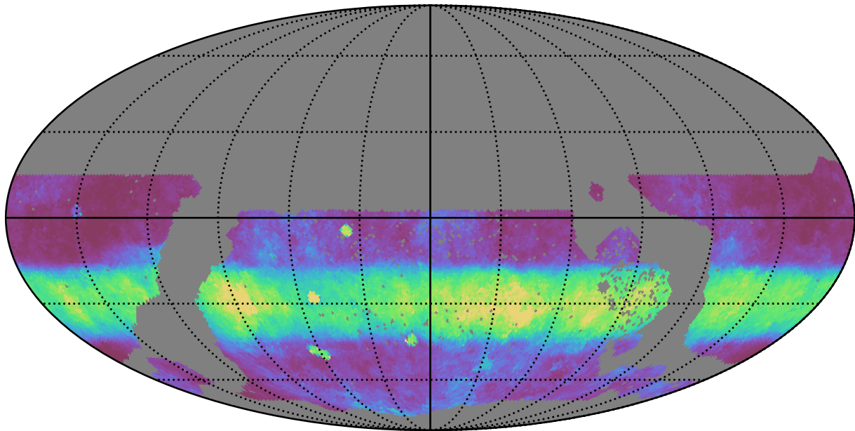
too_5_1v3.4_10yrs WFD i band: Median normairmass
