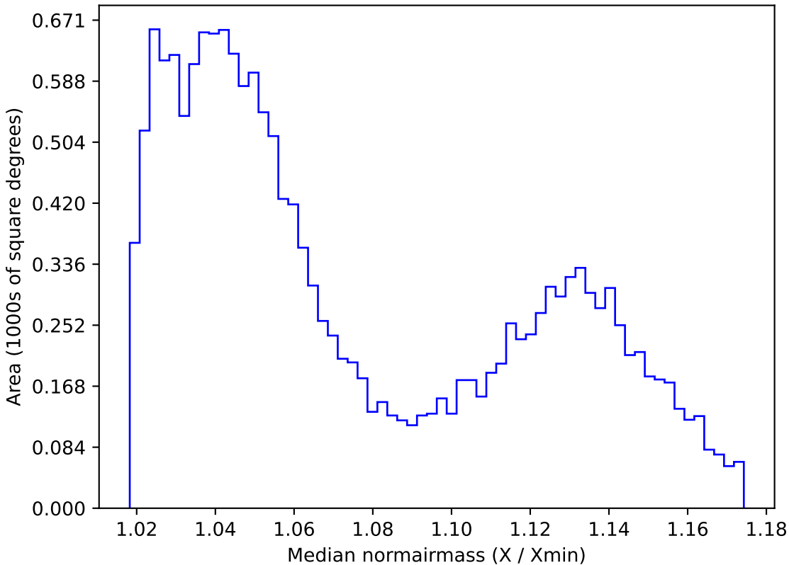
too_5_1v3.4_10yrs WFD i band: Median normairmass
