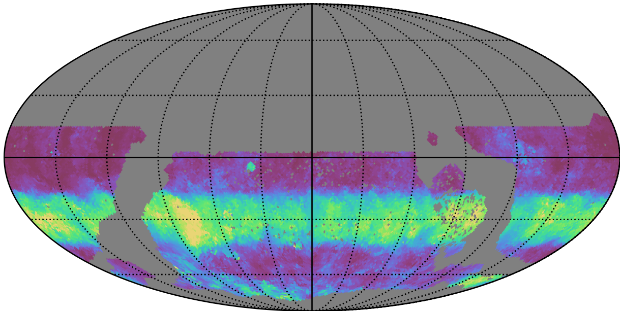
too_5_1v3.4_10yrs WFD g band: Median normairmass
