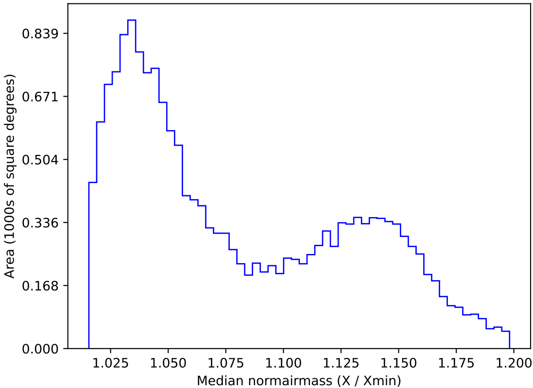
too_5_1v3.4_10yrs WFD g band: Median normairmass
