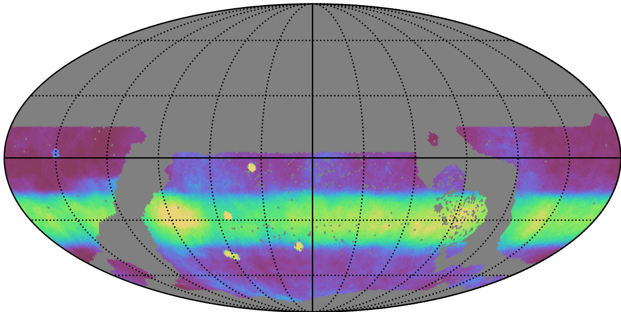
too_5_1v3.4_10yrs WFD all bands: Median normairmass
