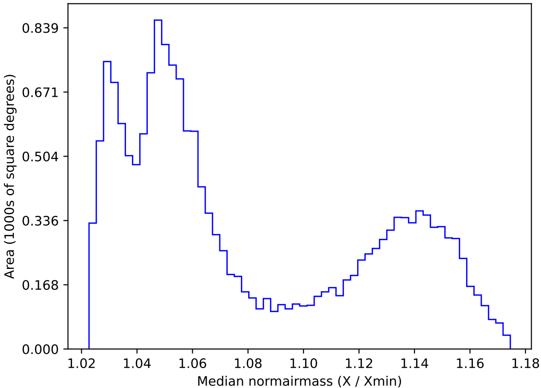
too_5_1v3.4_10yrs WFD all bands: Median normairmass
