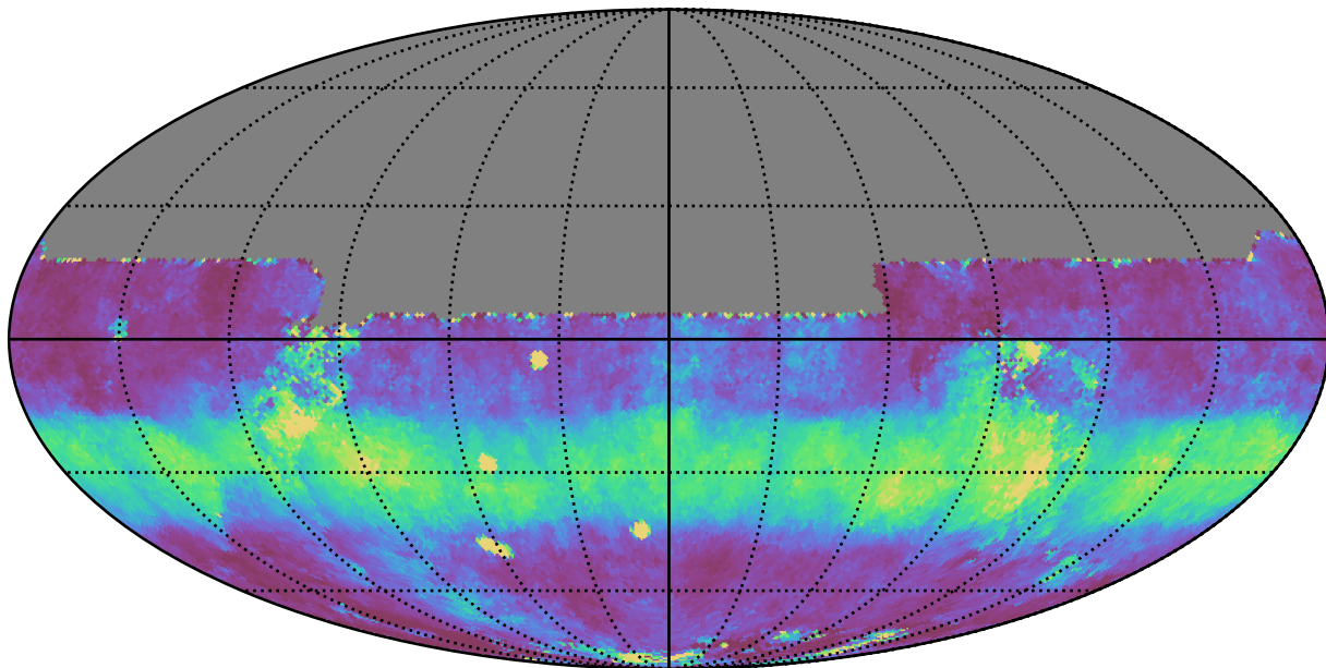
too_5_1v3.4_10yrs All sky y band: Median normairmass
