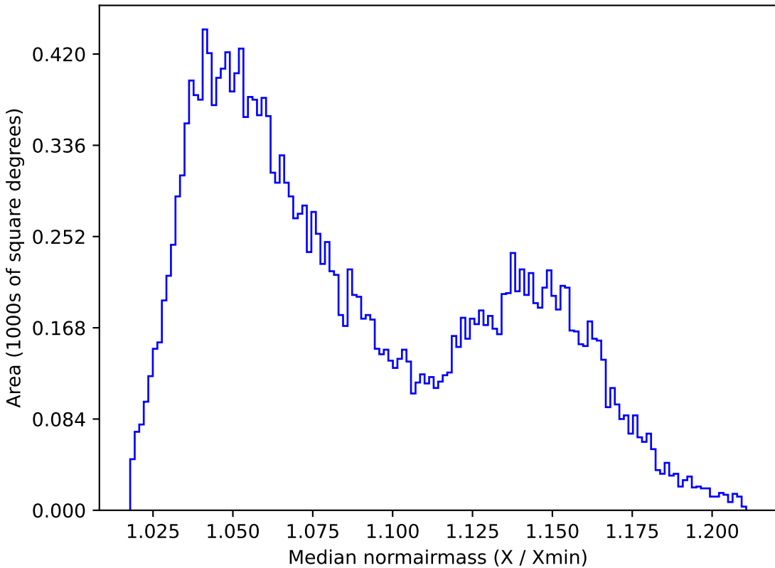
too_5_1v3.4_10yrs All sky y band: Median normairmass
