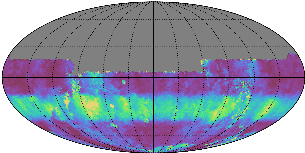
too_5_1v3.4_10yrs All sky u band: Median normairmass
