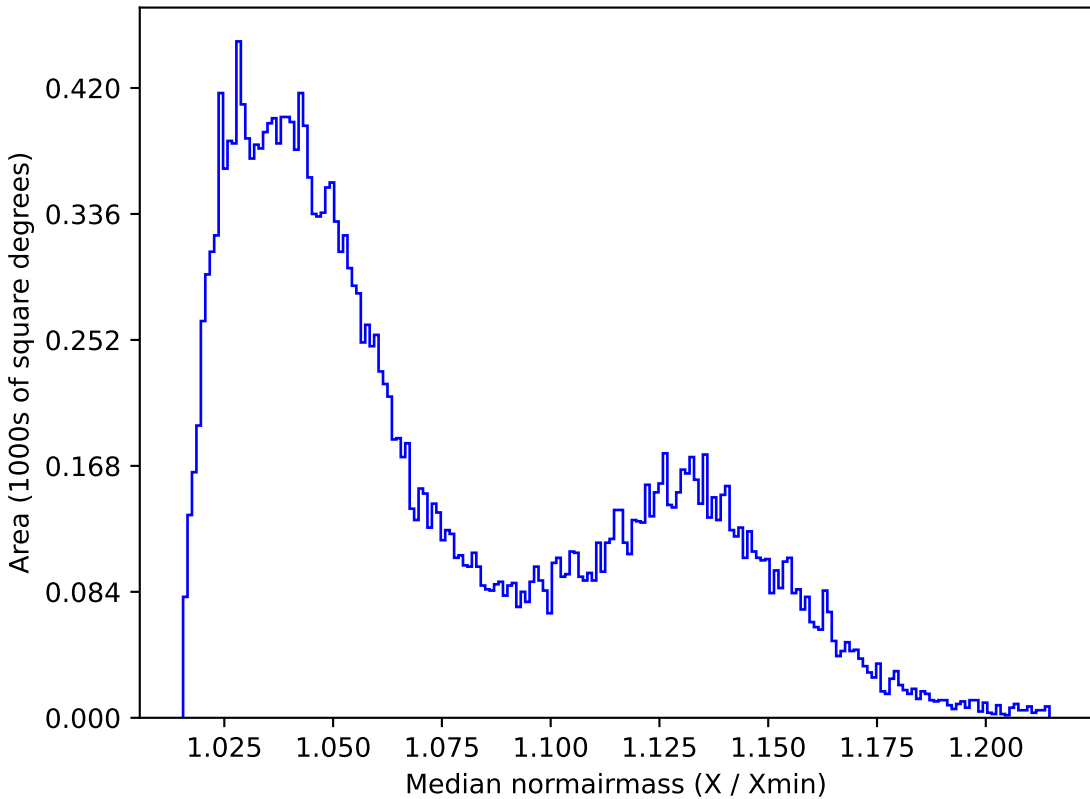
too_5_1v3.4_10yrs All sky i band: Median normairmass
