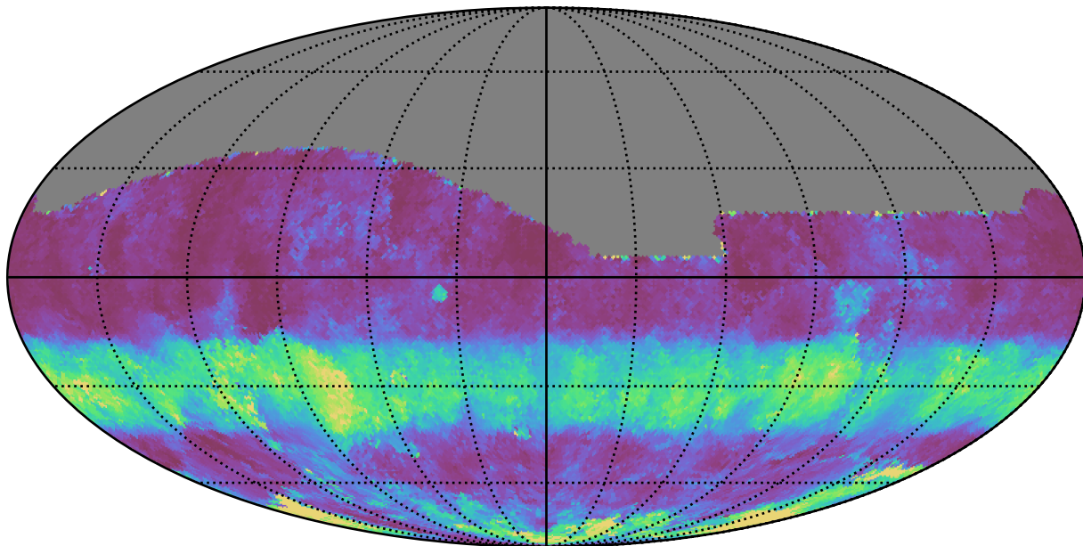
too_5_1v3.4_10yrs All sky g band: Median normairmass
