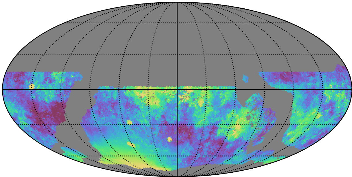
too_5_1v3.4_10yrs WFD z band: Median moonDistance
