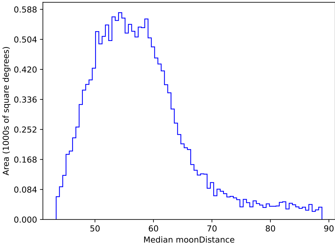
too_5_1v3.4_10yrs WFD y band: Median moonDistance
