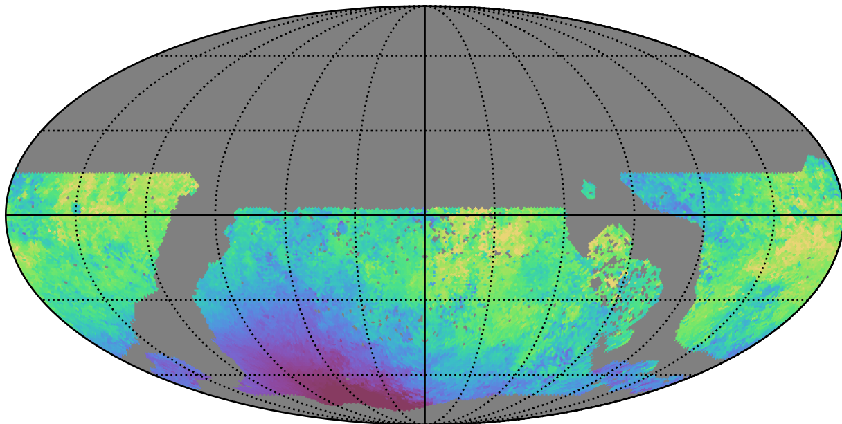
too_5_1v3.4_10yrs WFD u band: Median moonDistance
