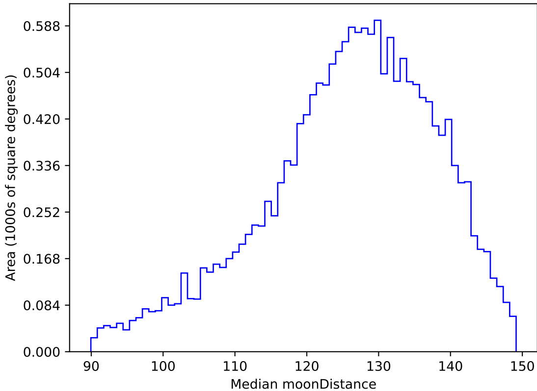
too_5_1v3.4_10yrs WFD u band: Median moonDistance
