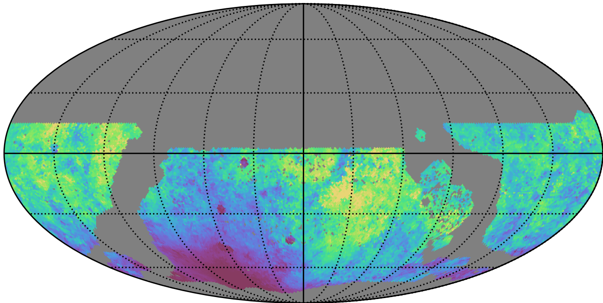
too_5_1v3.4_10yrs WFD r band: Median moonDistance
