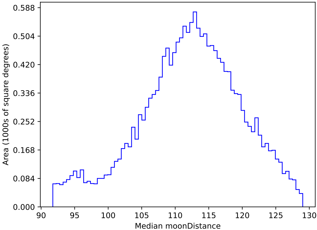
too_5_1v3.4_10yrs WFD r band: Median moonDistance
