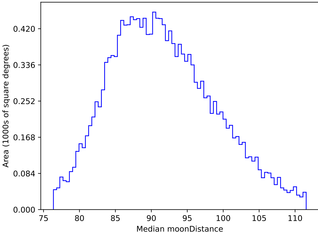
too_5_1v3.4_10yrs WFD i band: Median moonDistance
