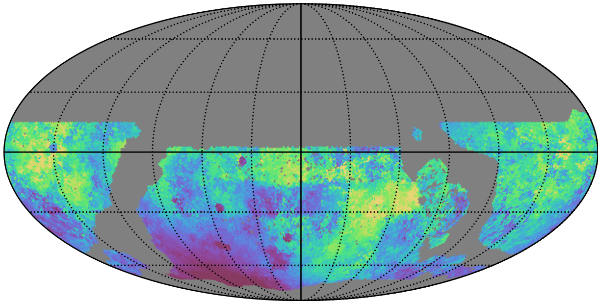
too_5_1v3.4_10yrs WFD g band: Median moonDistance
