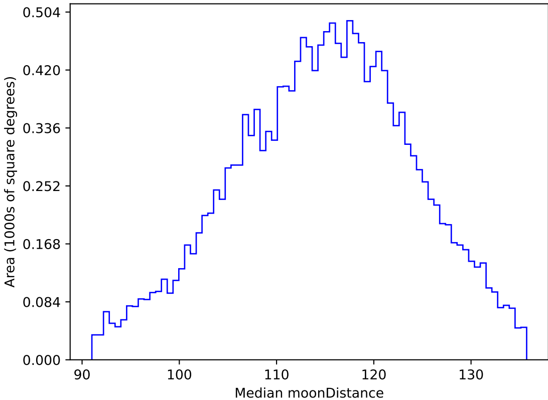
too_5_1v3.4_10yrs WFD g band: Median moonDistance
