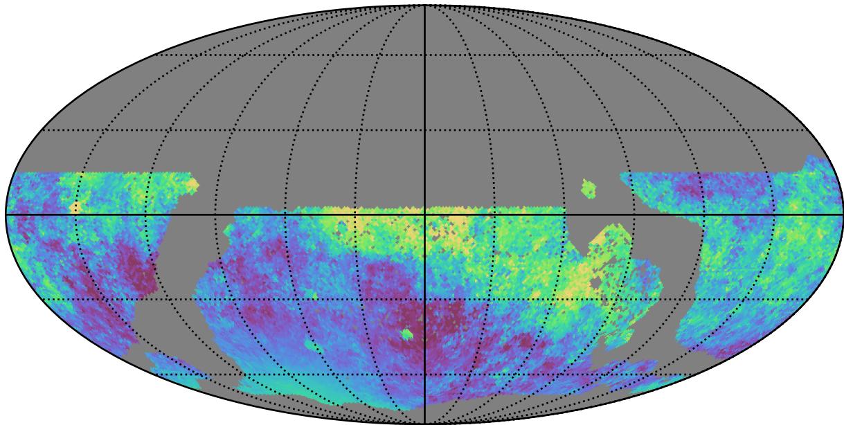
too_5_1v3.4_10yrs WFD all bands: Median moonDistance
