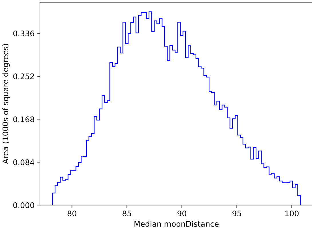
too_5_1v3.4_10yrs WFD all bands: Median moonDistance
