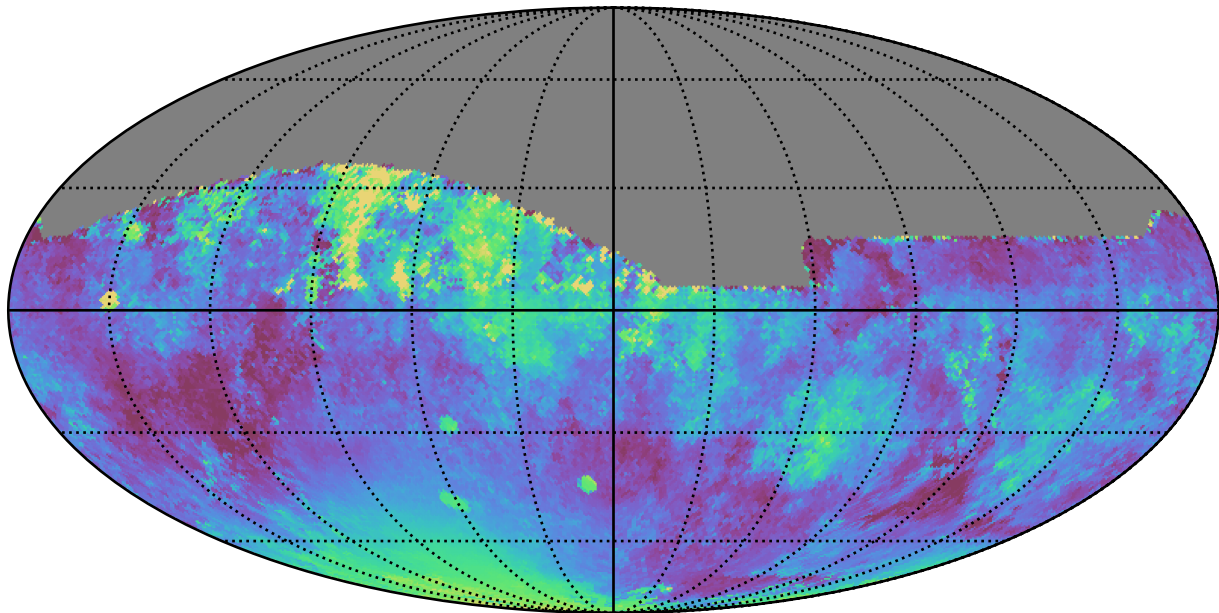
too_5_1v3.4_10yrs All sky z band: Median moonDistance
