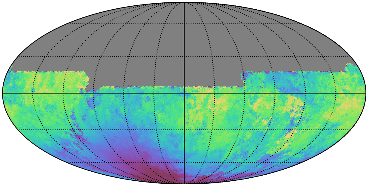
too_5_1v3.4_10yrs All sky u band: Median moonDistance
