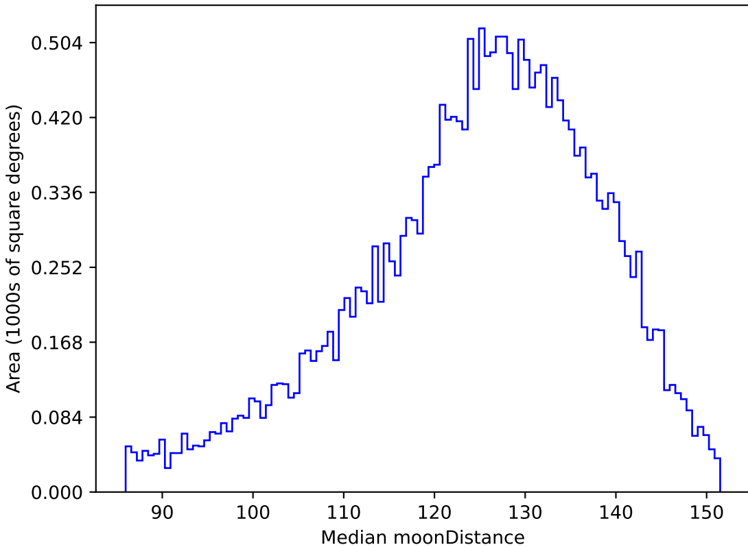
too_5_1v3.4_10yrs All sky u band: Median moonDistance
