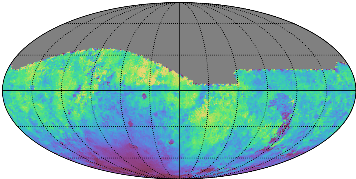
too_5_1v3.4_10yrs All sky r band: Median moonDistance
